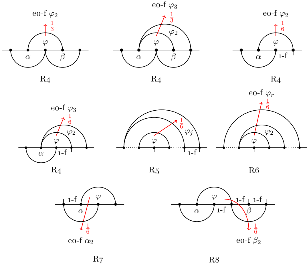
Figure 8.2: Redistribution rules R_4 – R_8 ( 1\text{-}f is a 1-face and eo\text{-}f is an empty o-face).
